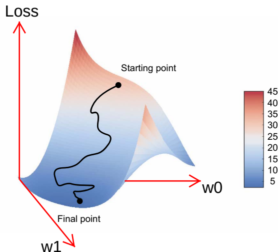
Figure 2.19 Gradient descent down a 2D loss surface (two learnable parameters)
